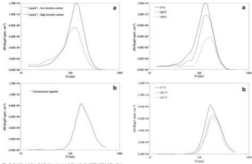
Fig. 3. Particle number distribution measured through the PMPS 3001 (after thermodilution at 37 °C) of the mainstream aerosol from the Liquid 1 (a) and from the conventional tobacco cigarette (b).
